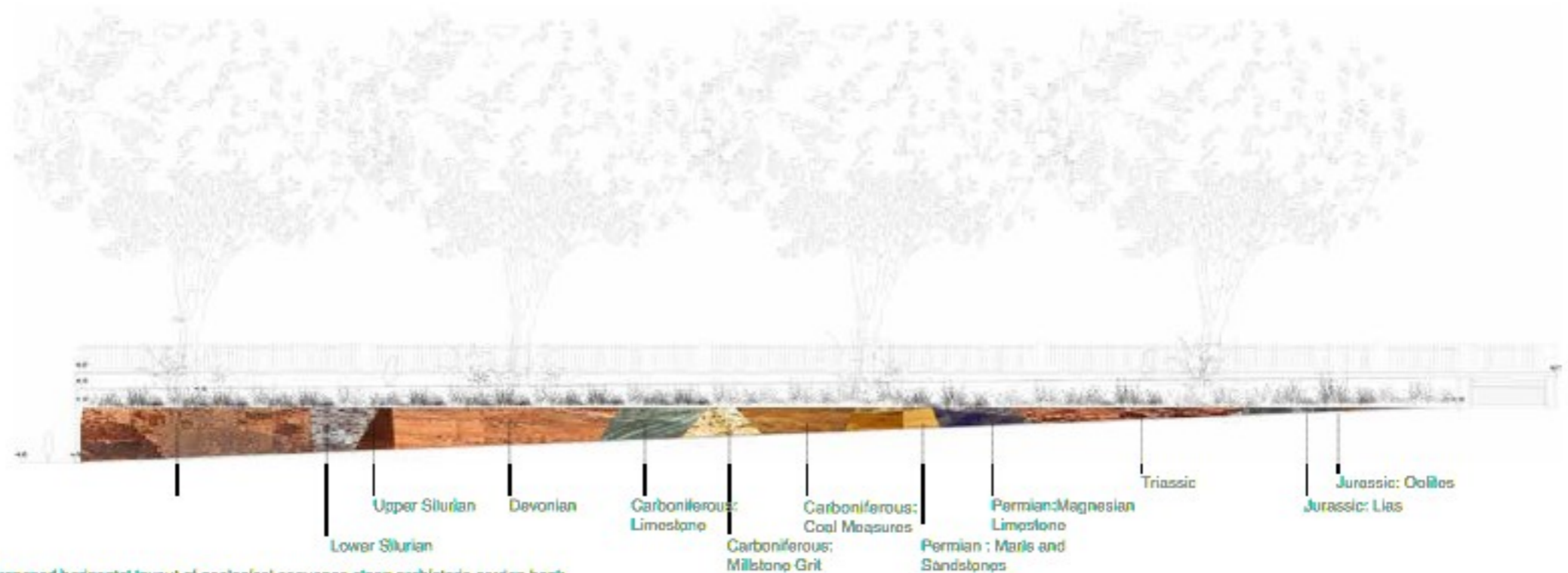
Proposed horizontal layout of geological sequence along prehistoric garden bank
