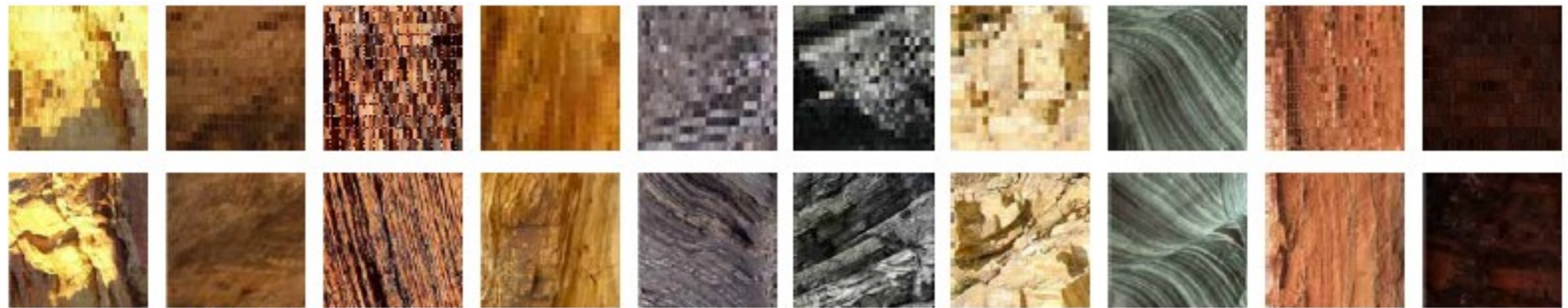
Concept images of rock patterns in the British Isles
